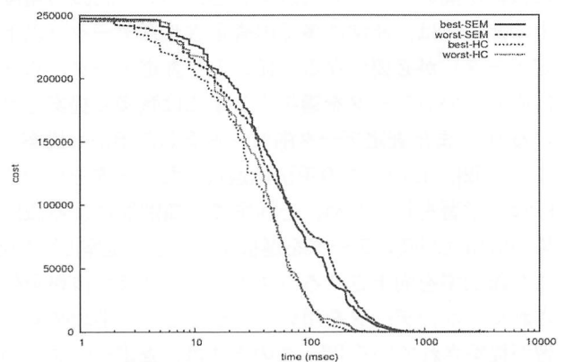
Fig.1. Comparison of the computational time, n=500
