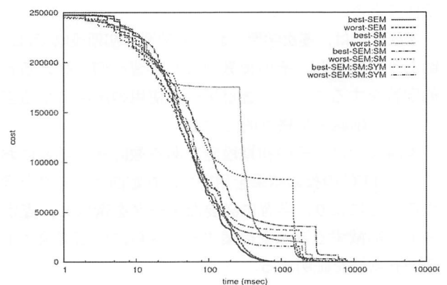
Fig.2. Comparison of the computational time, n=500
